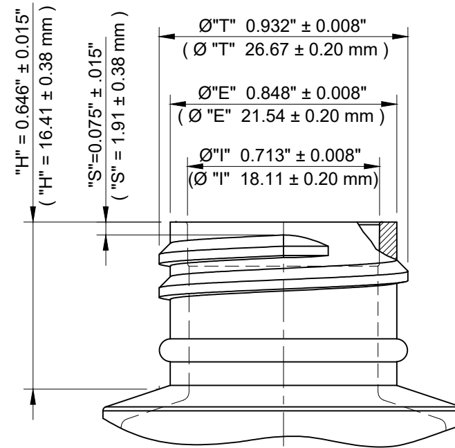
NECK DETAIL
