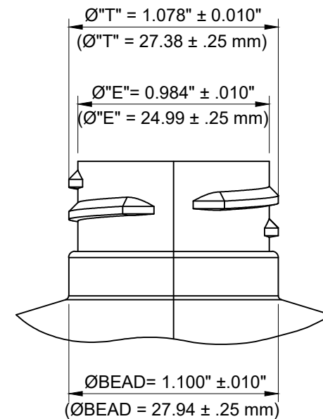
NECK DETAIL
