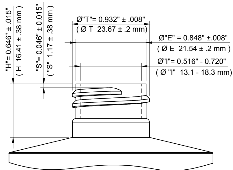
NECK DETAIL
